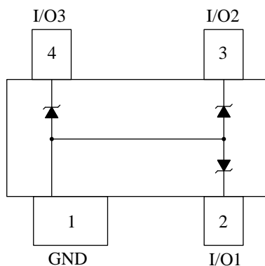
Circuit Diagram and Pin Schematic
